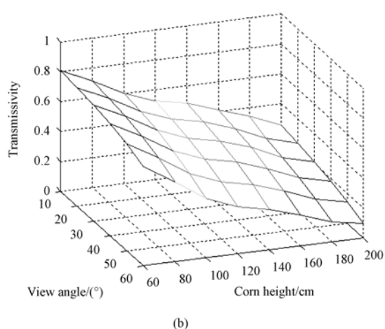
Fig. 8 (a) Effective single scattering albedo of corn at X-band and V pol. vs. view angle and height; (b) Transmissivity of corn at X-band and H pol. vs. view angle and height
