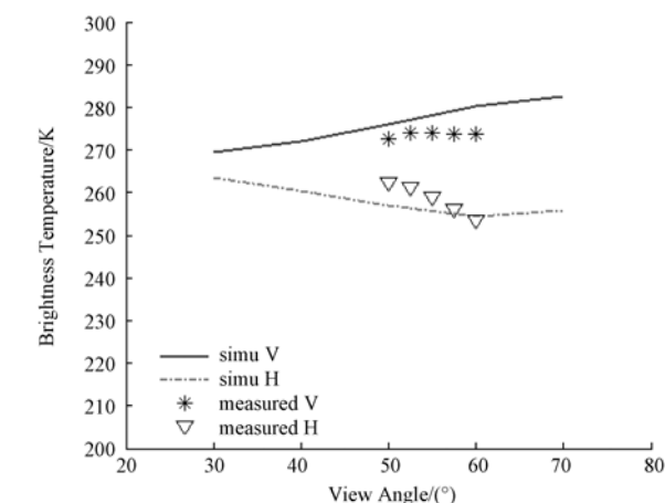
Fig. 5 Comparison of simulation and measured Brightness Temperature at 6.925GHz (80% cover)
